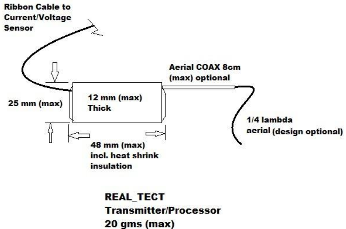
Figure 2 REAL-TECT TRANSMITTER/PROCESSOR
